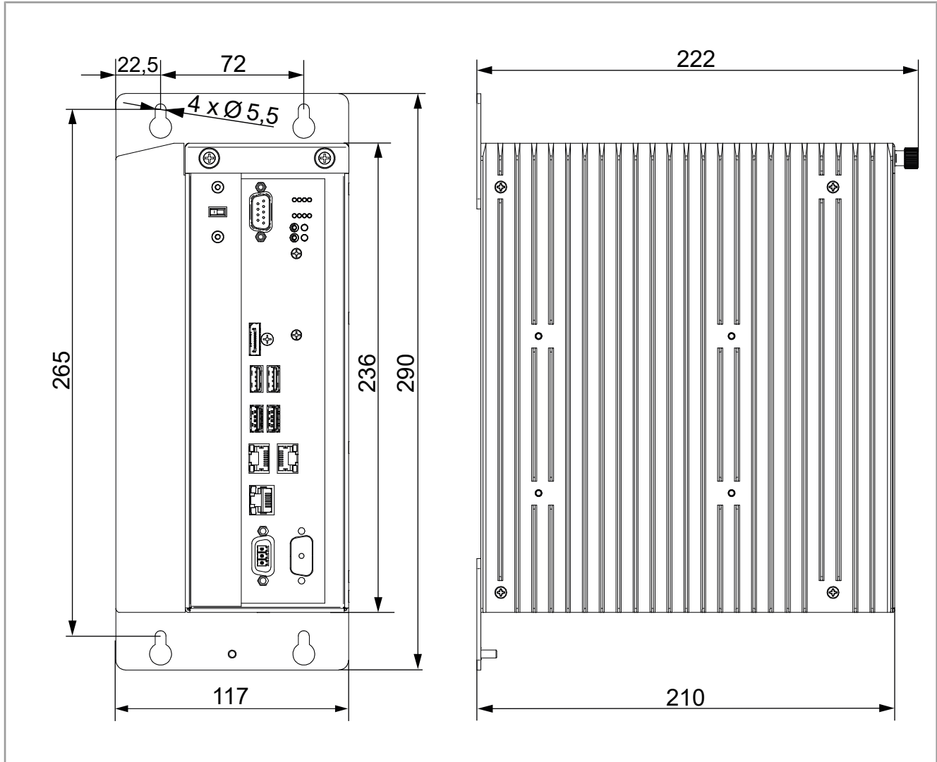
Abb. 6: Abmessungen in mm
