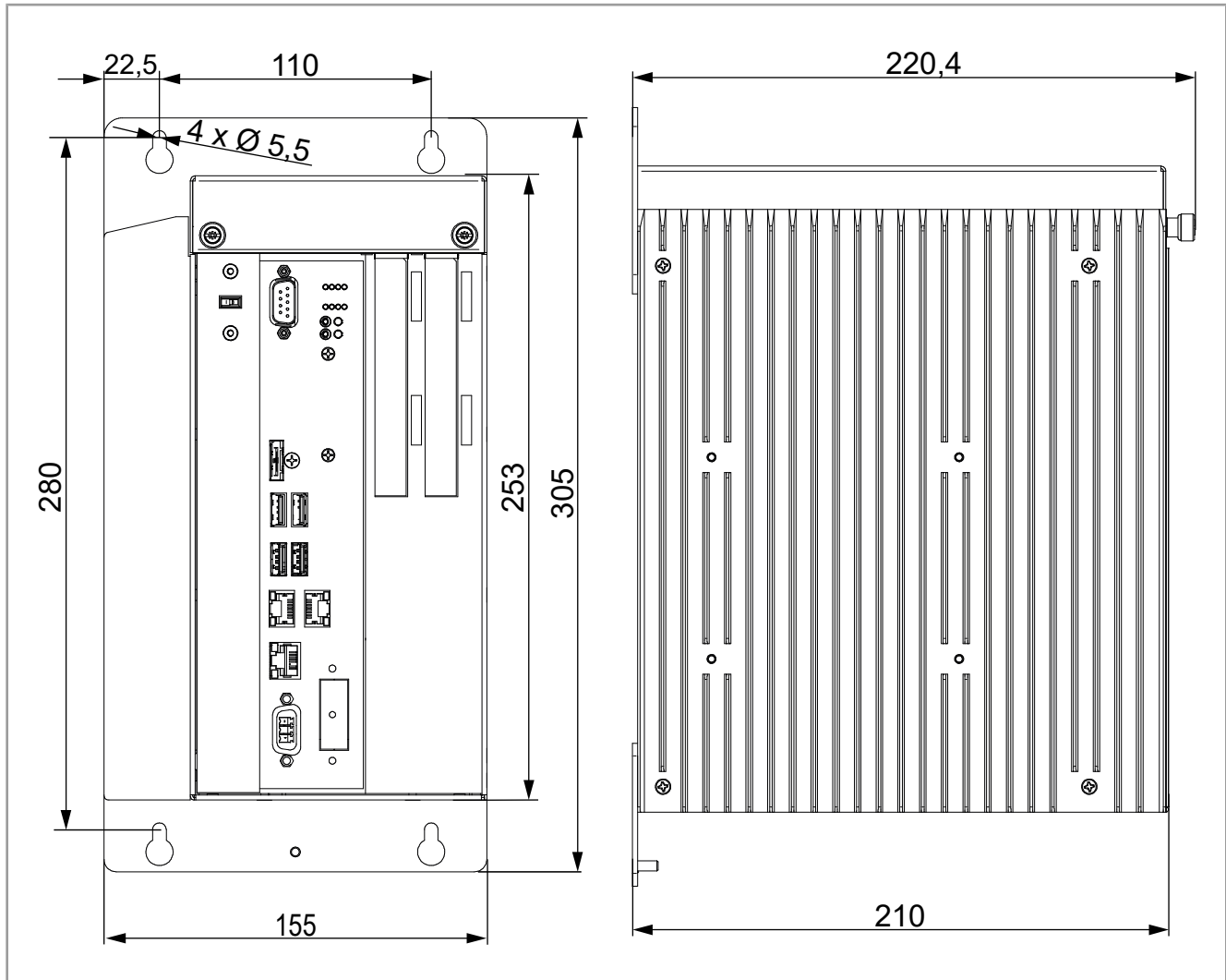
Abb. 6: Abmessungen in mm
